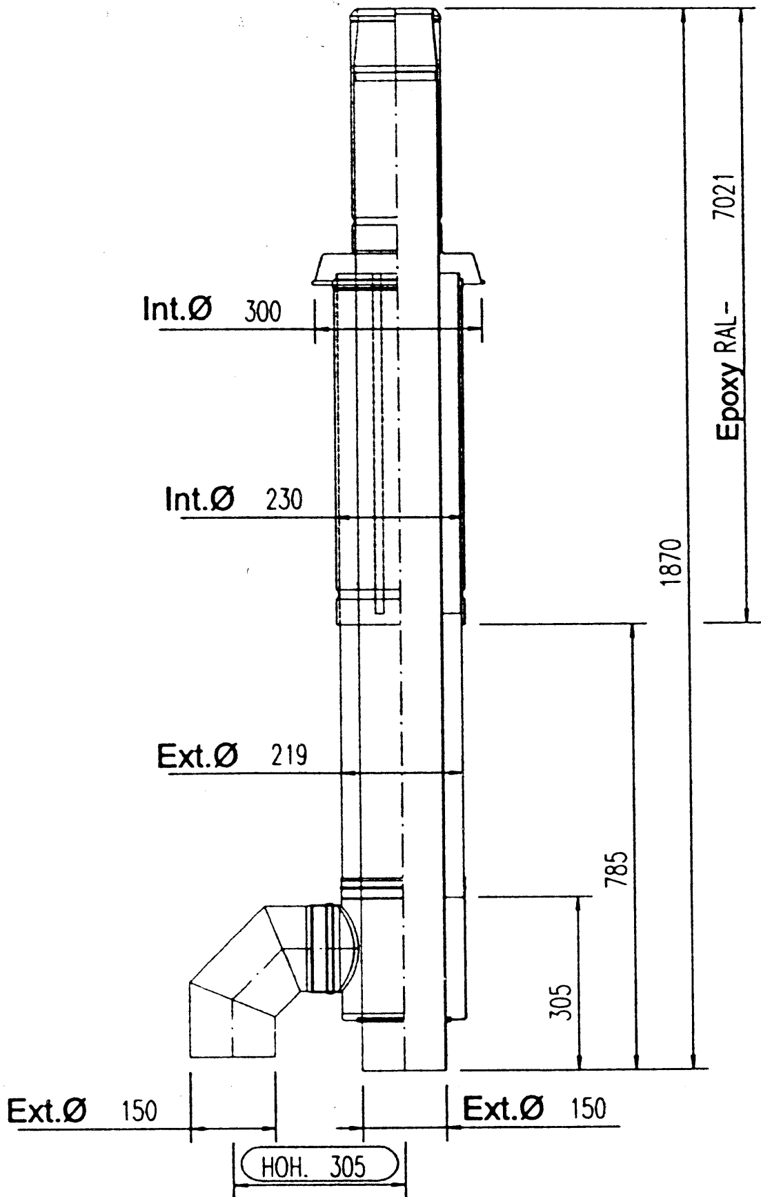
Fig. 12 Vertical terminal for room sealed operation
